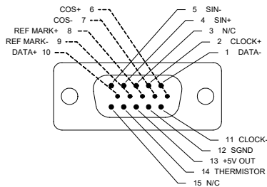
Absolute Encoder
