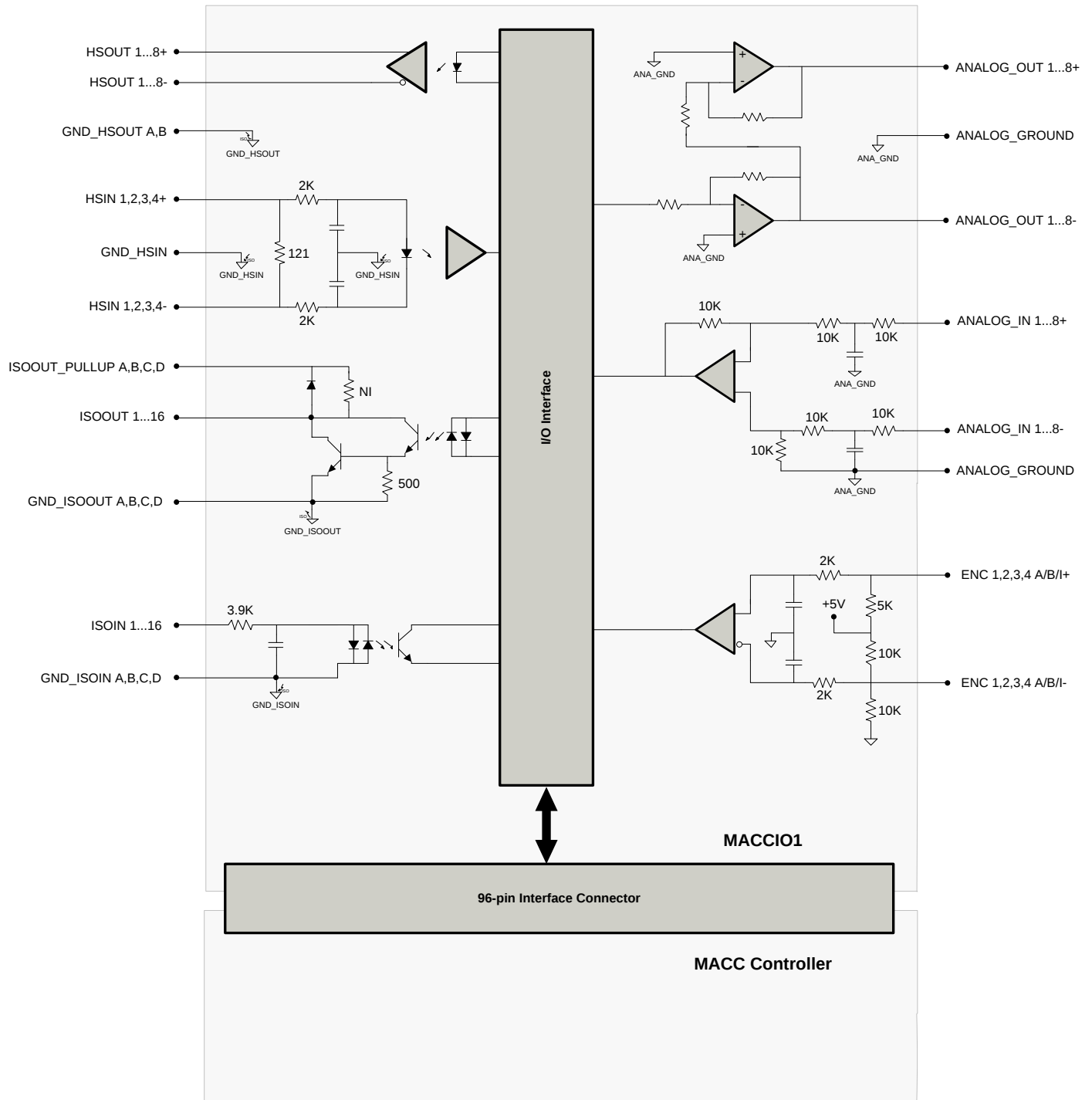
Galvanically Isolated High-Speed I/O Board Population Option
